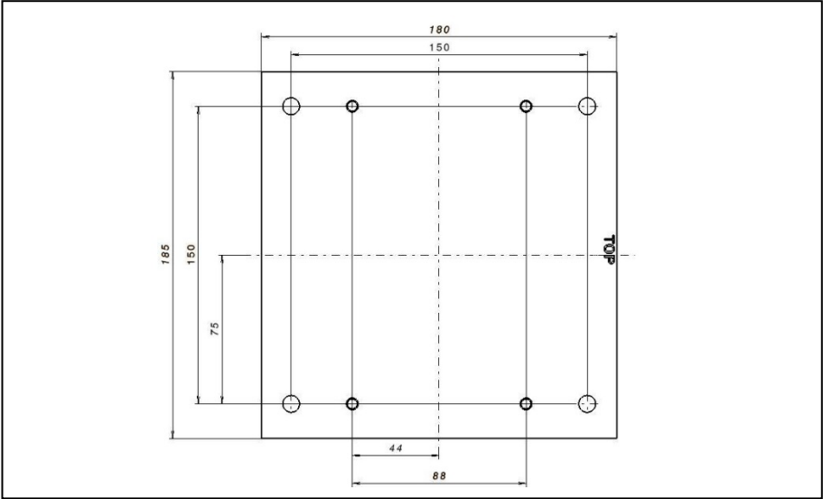
Abb. 56: Bohrbild Standard-Wand-Adapterplatte BG D
